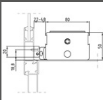
On windows with windowsill without brackets
