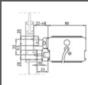
Without windowsill with bracket part No. 40460N
